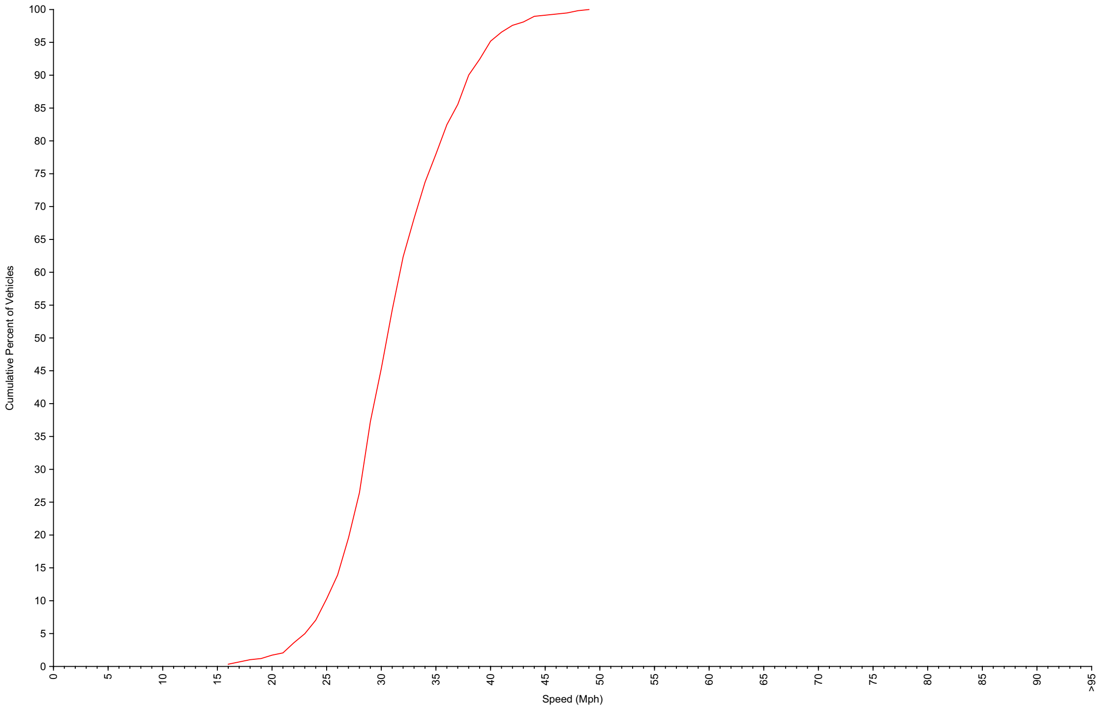
Cumulative Speed Distribution Curve Daily Overview for Sat Oct 21 2023
