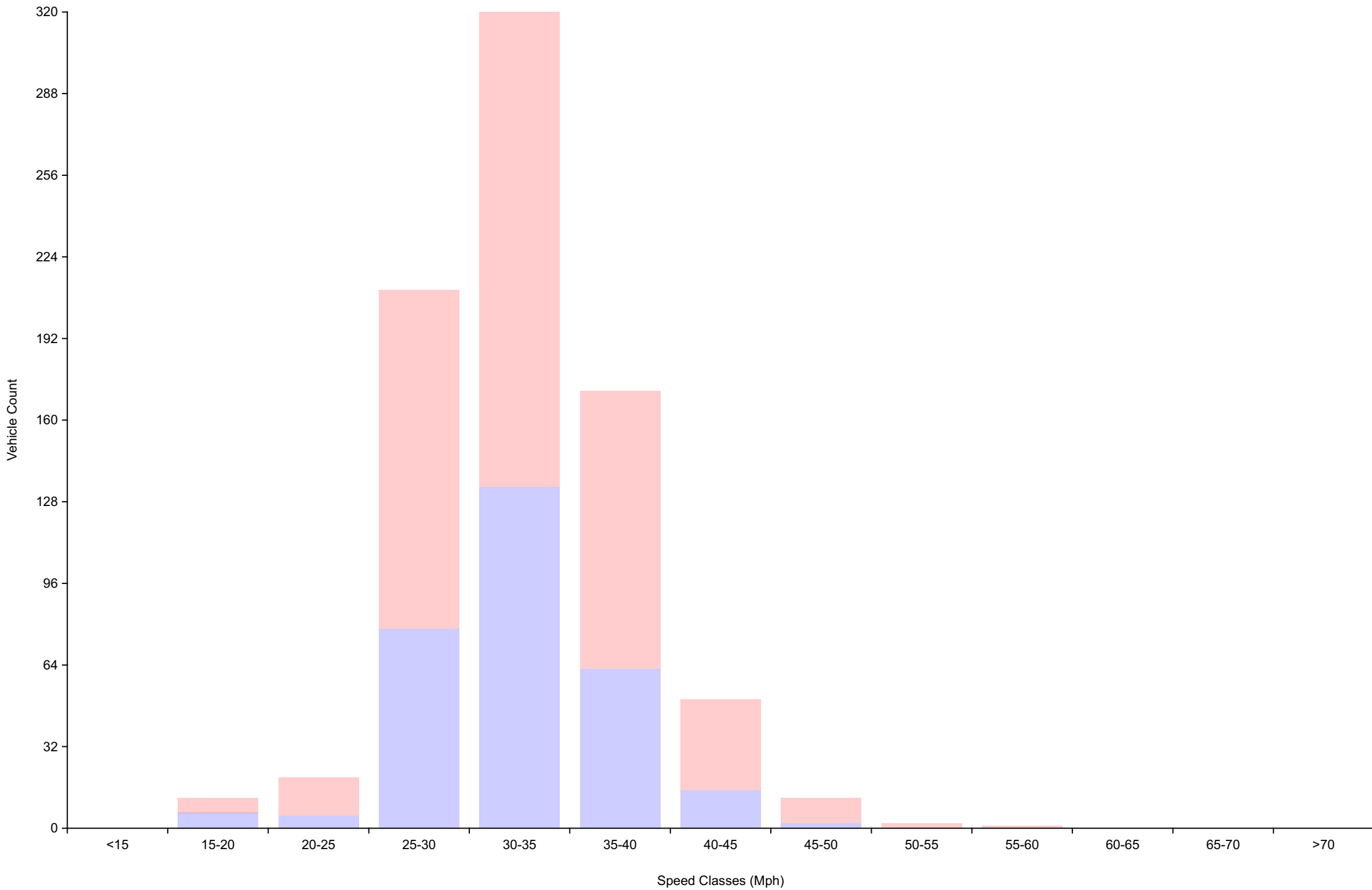
Vehicle Counts By Speed Class Daily Overview for Tue Oct 17 2023
