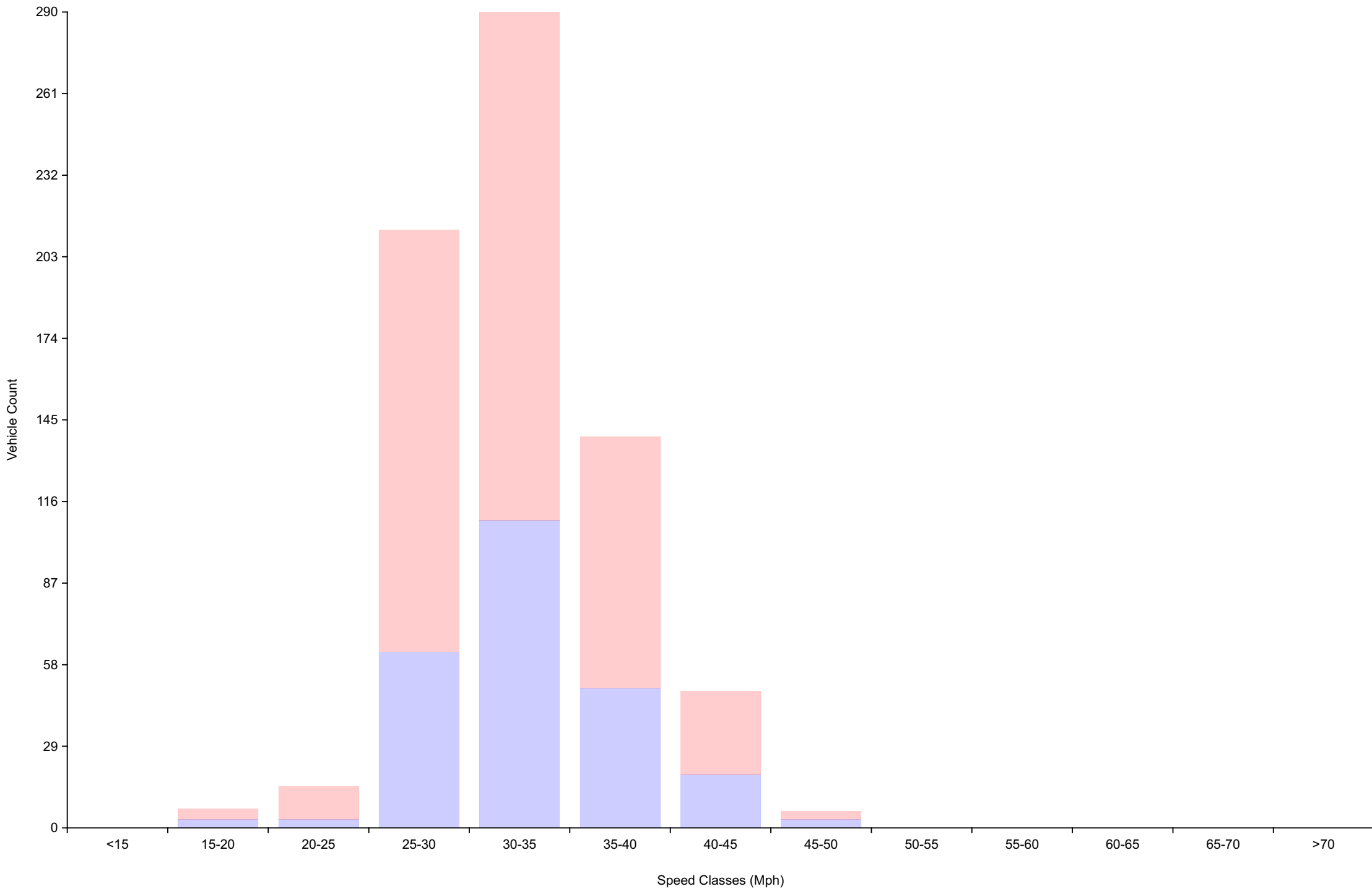
Vehicle Counts By Speed Class Daily Overview for Mon Oct 23 2023
