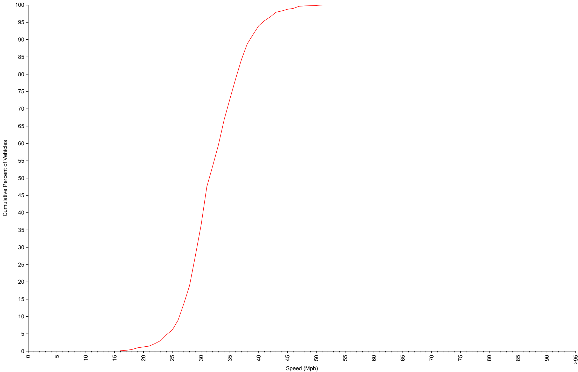
Cumulative Speed Distribution Curve Daily Overview for Wed Oct 18 2023
