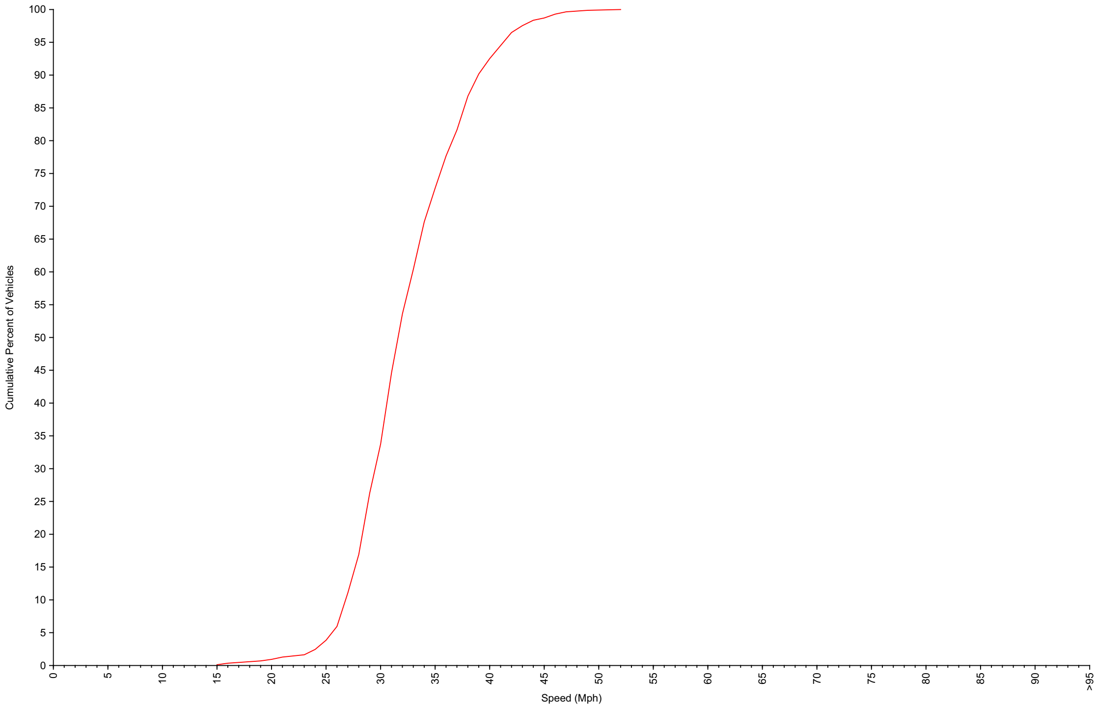
Cumulative Speed Distribution Curve Daily Overview for Wed Oct 11 2023
