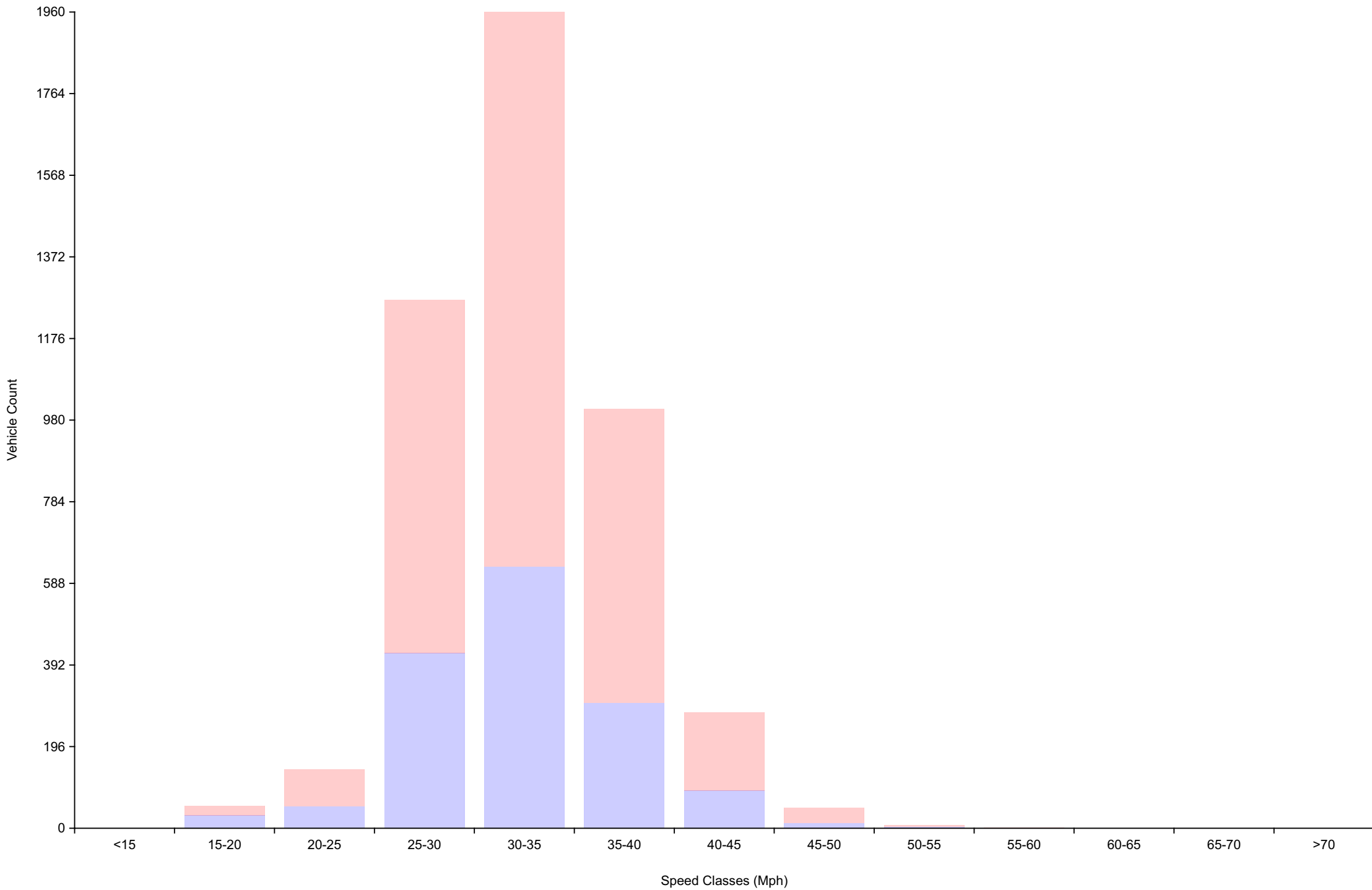
Vehicle Counts By Speed Class For week beginning Mon Oct 16 2023
