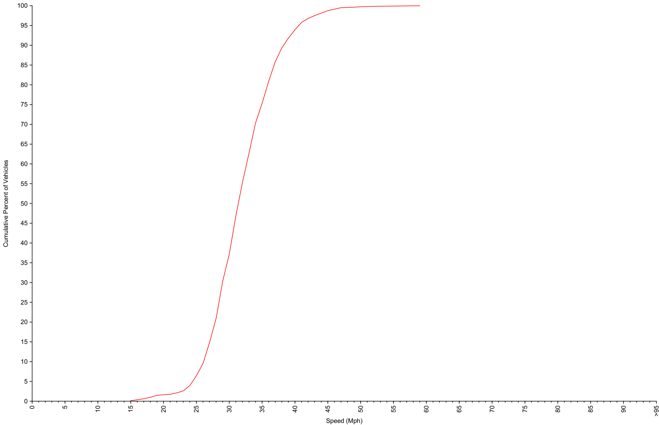
Cumulative Speed Distribution Curve Daily Overview for Tue Oct 17 2023
