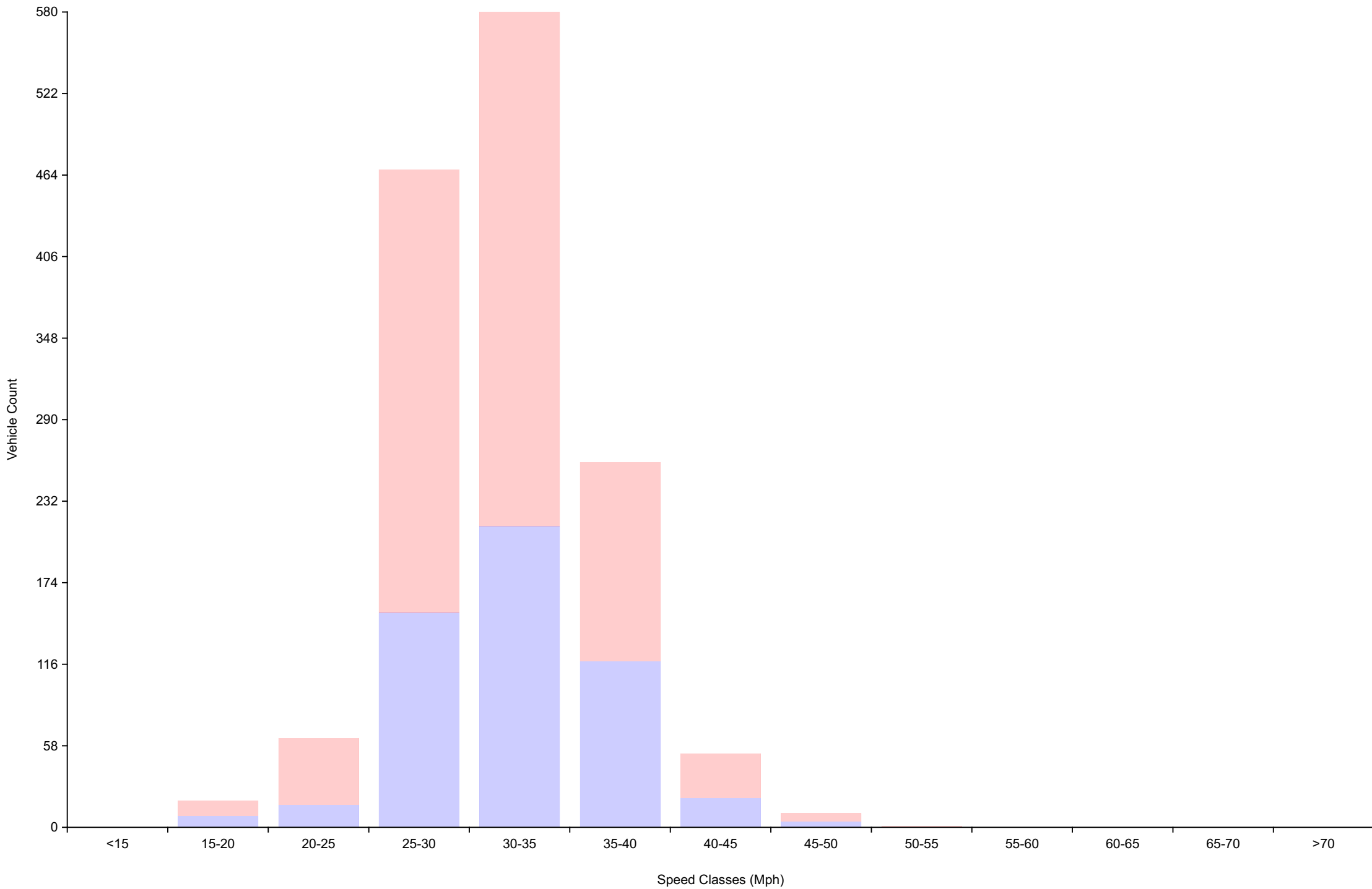
Vehicle Counts By Speed Class For week beginning Mon Oct 30 2023
