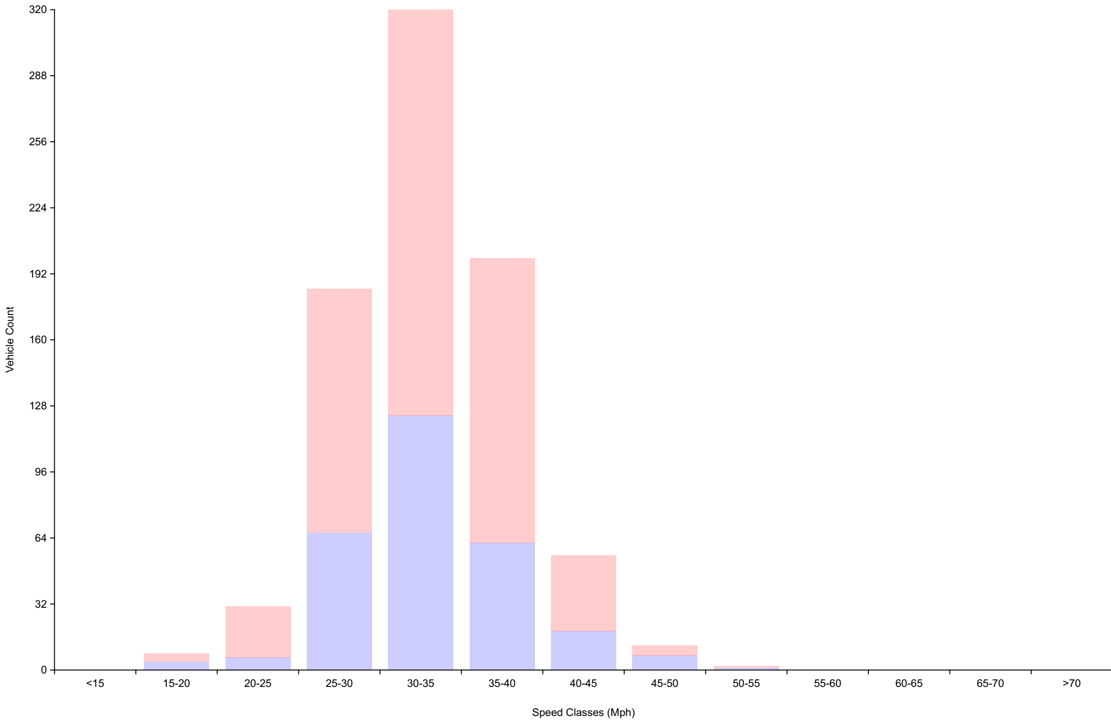
Vehicle Counts By Speed Class Daily Overview for Wed Oct 18 2023
