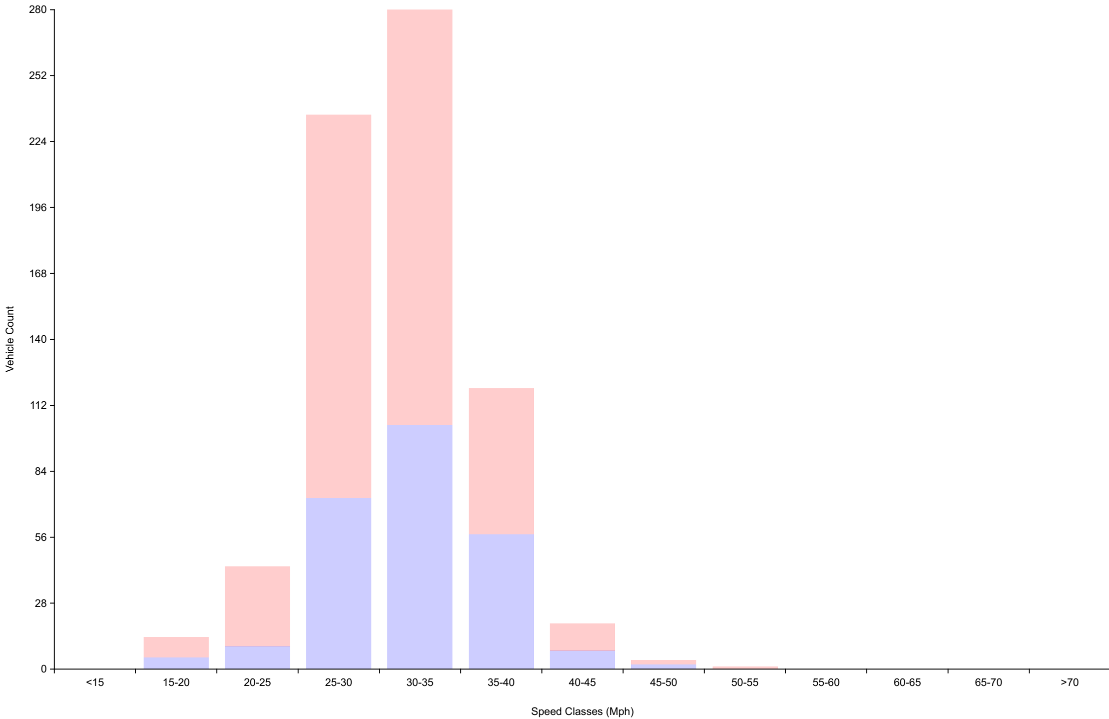
Vehicle Counts By Speed Class Daily Overview for Tue Oct 31 2023
