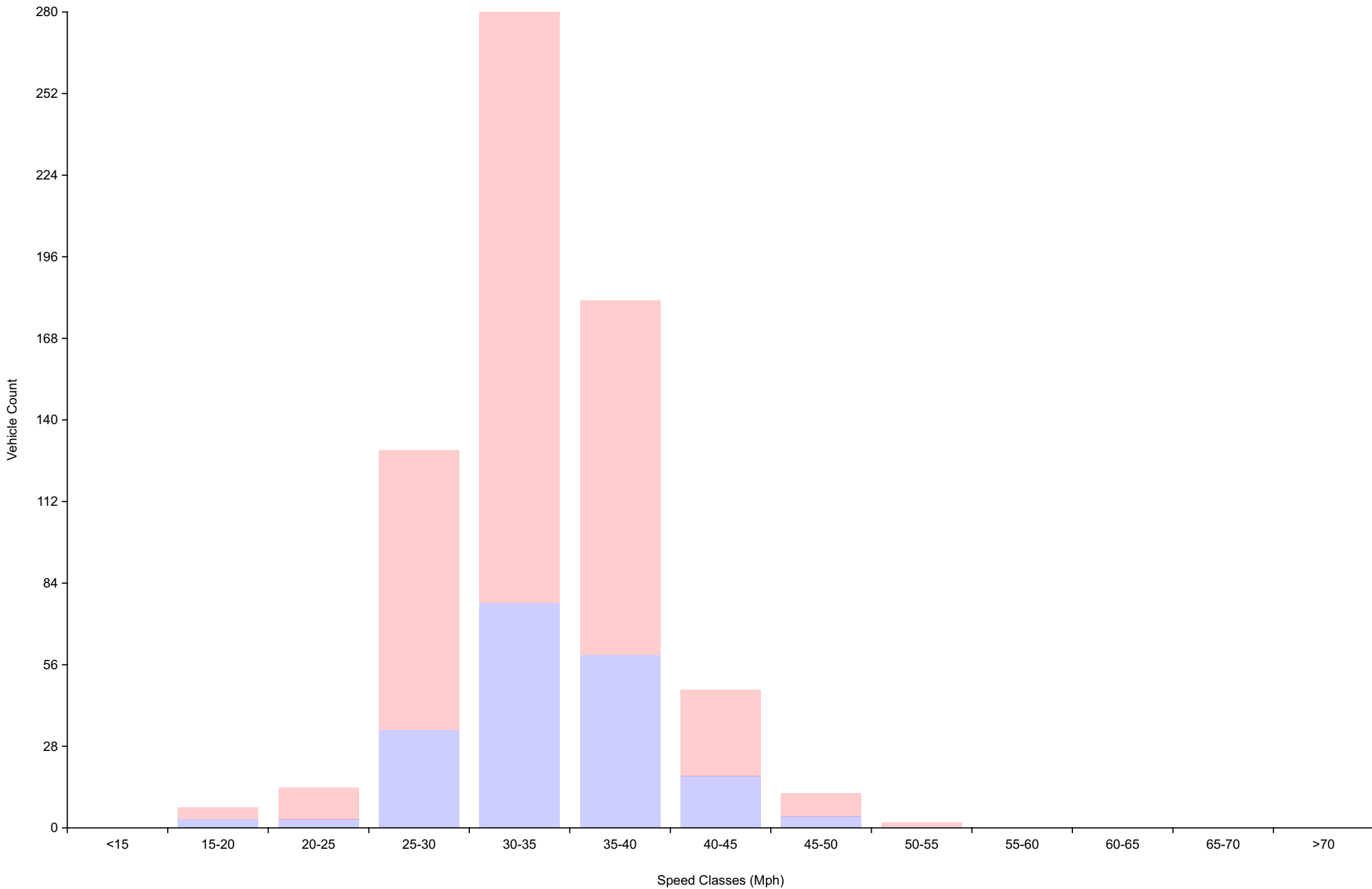
Vehicle Counts By Speed Class Daily Overview for Sat Oct 14 2023
