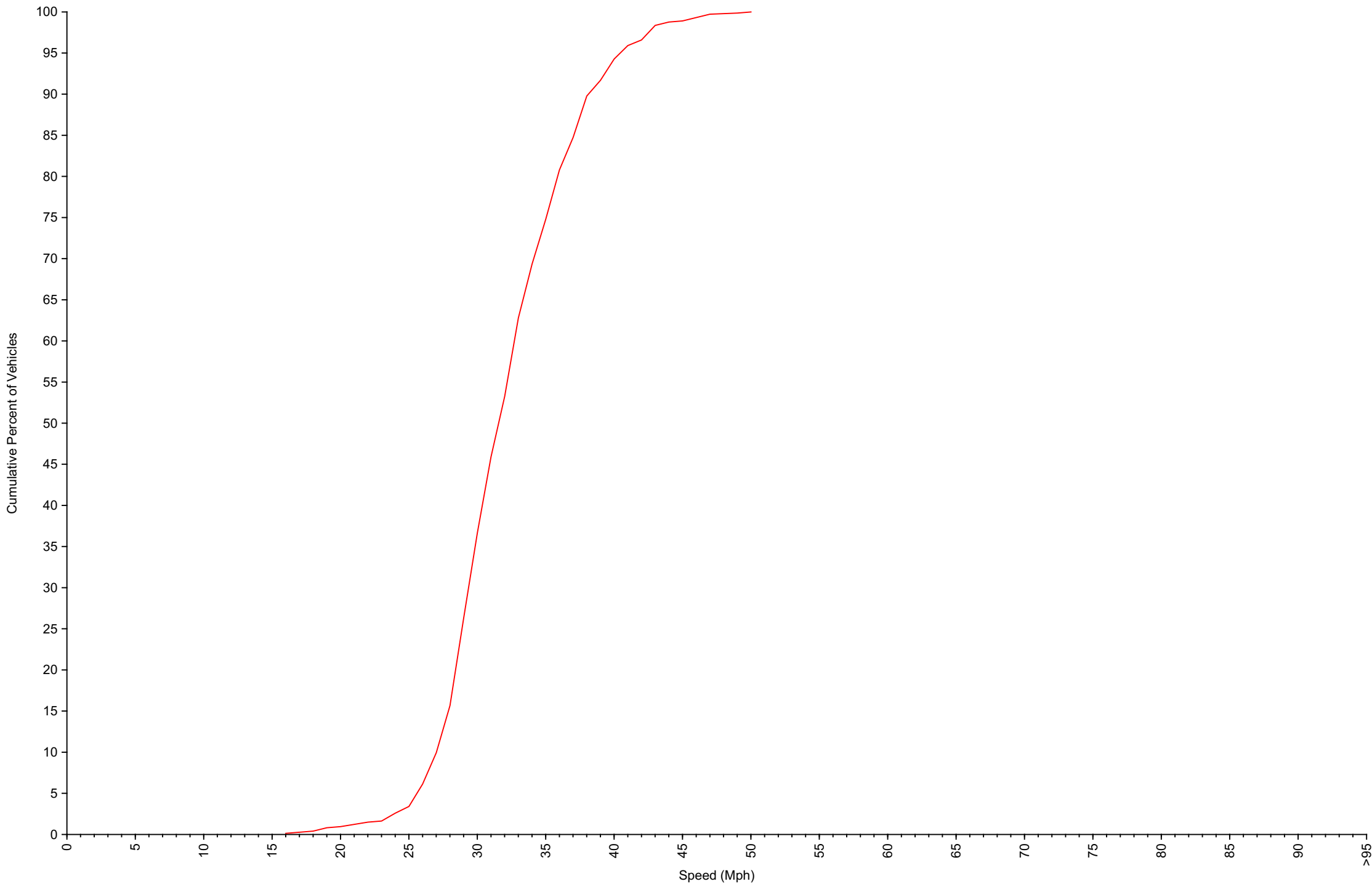
Cumulative Speed Distribution Curve Daily Overview for Mon Oct 16 2023
