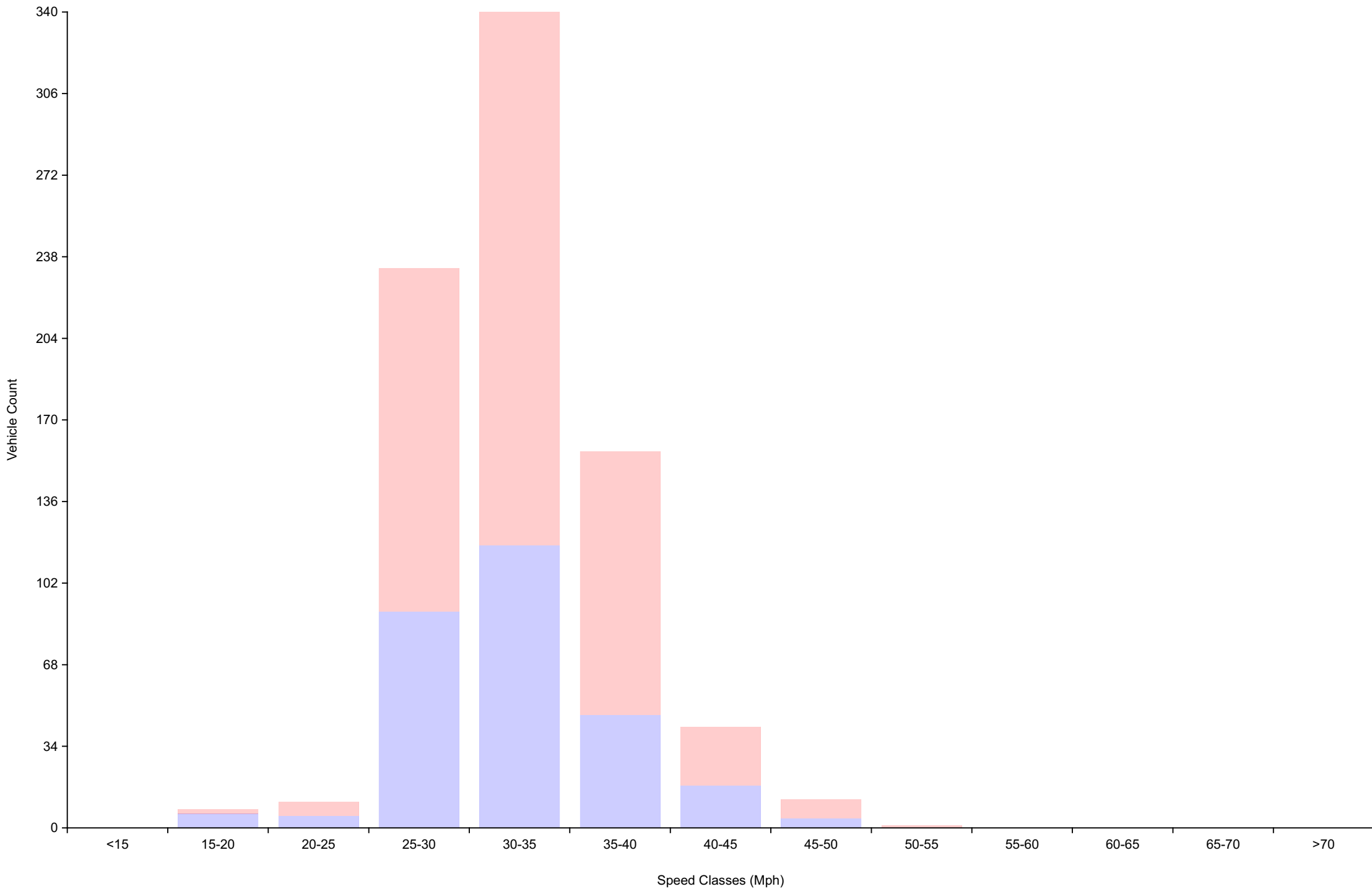
Vehicle Counts By Speed Class Daily Overview for Wed Oct 25 2023
