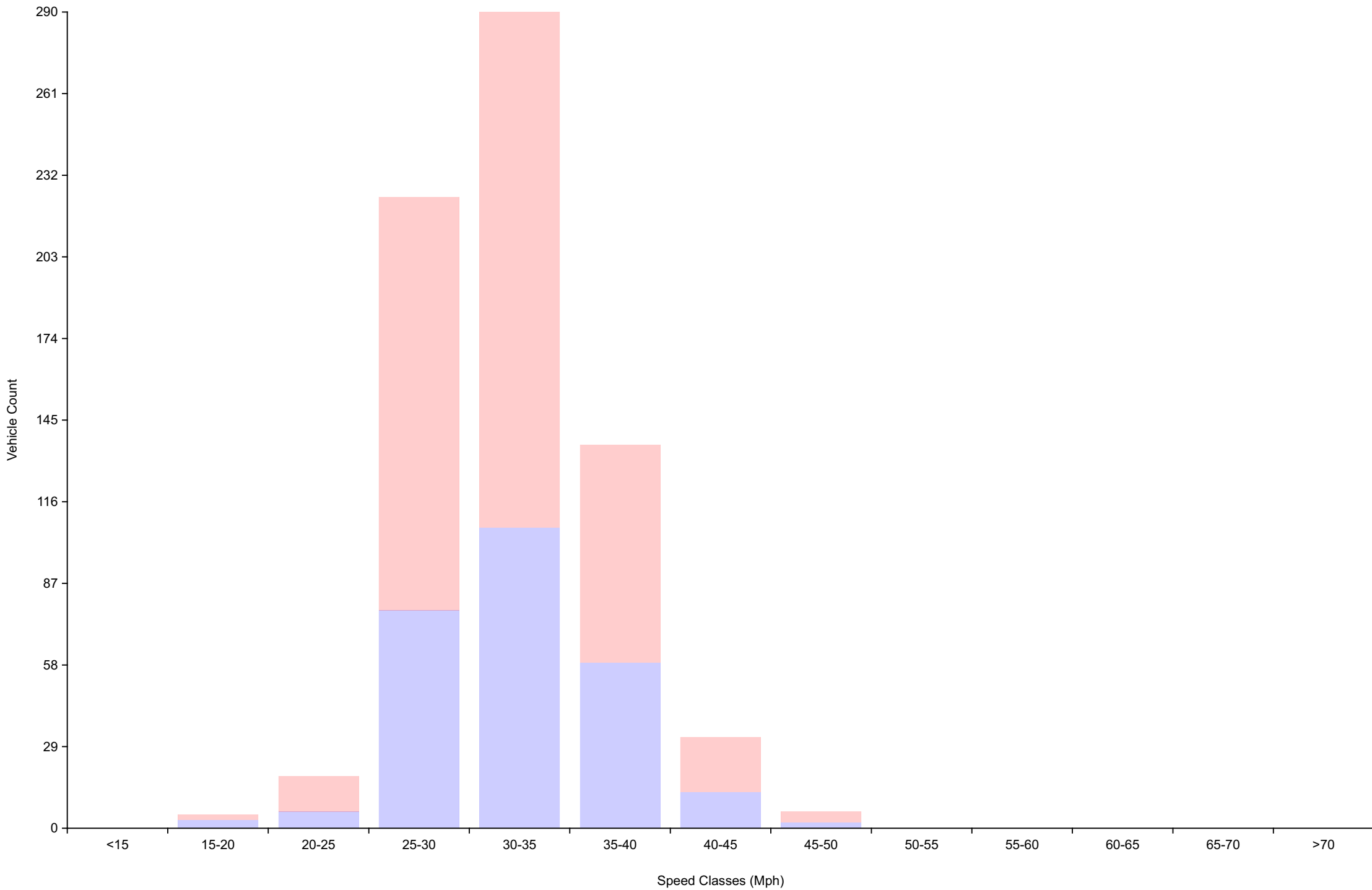
Vehicle Counts By Speed Class Daily Overview for Mon Oct 30 2023
