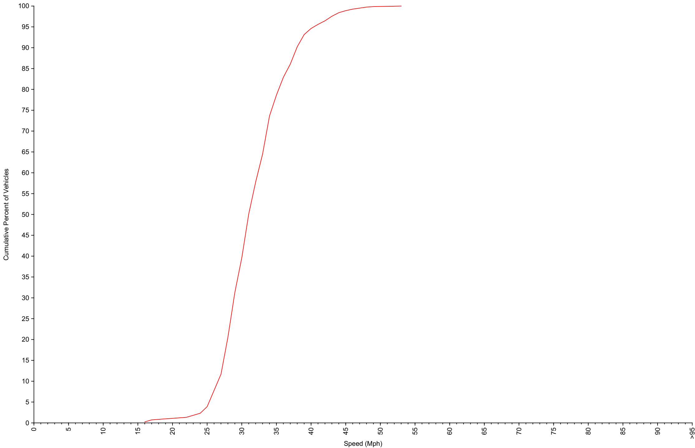
Cumulative Speed Distribution Curve Daily Overview for Wed Oct 25 2023
